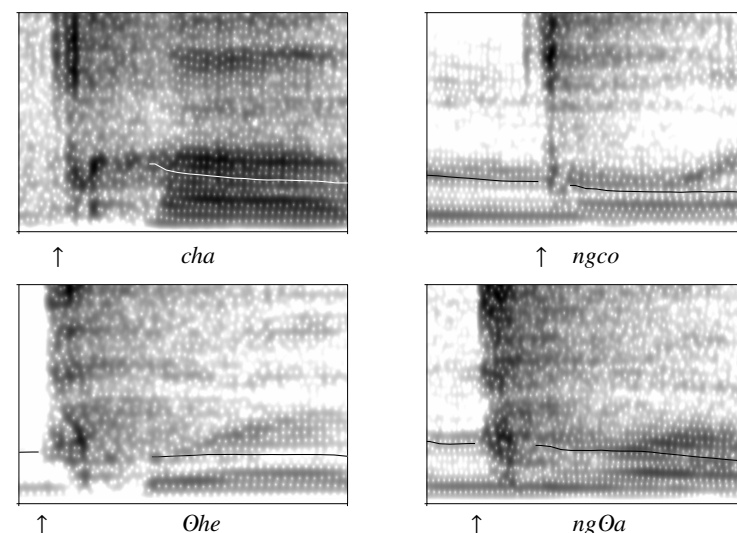
Productions of native (top row) and novel (bottom row) aspirated and breathy nasal clicks, from the orthographically presented words ukuchaza , ukuǀhele , ukungcola , ingǀabha . Spectrogram y-axis from 0 to 5 kHz. Pitch contour marked, with y-axis from 75 to 500 Hz. Samples are 250–400 ms wide; the location of the click burst is marked. The pitch contour interruption in the breathy nasals is probably the analysis being overwhelmed by the click burst. Analysis and rendering by Praat (Boersma and Weenink 2013).
